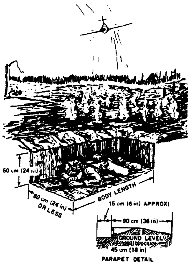
Figure 1-5. Prone emplacement.
